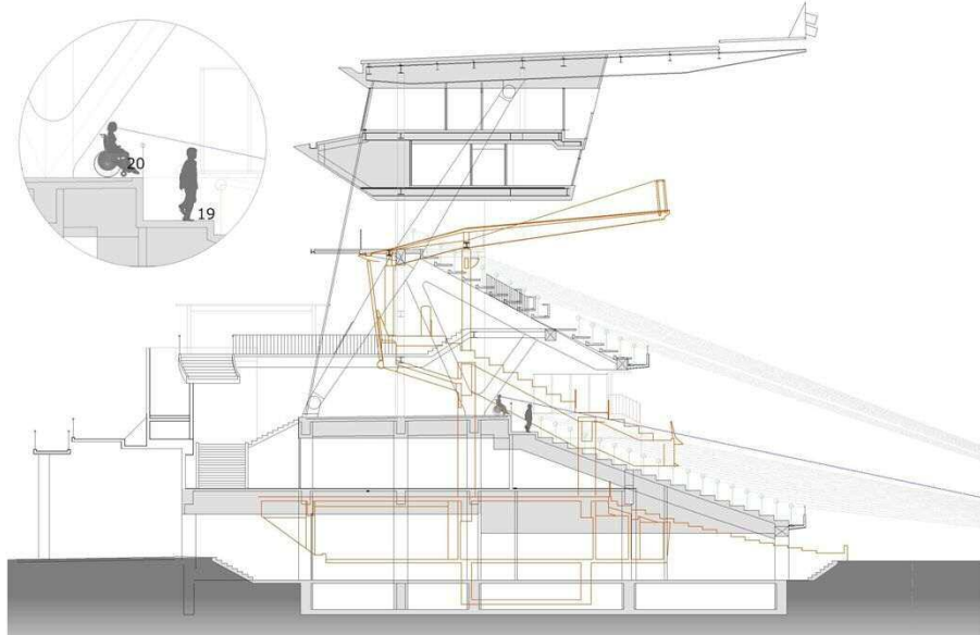
Reconstruction Work of Todoroki Stadium Grandstand
