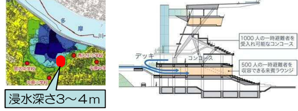
Reconstruction Work of Todoroki Stadium Grandstand
